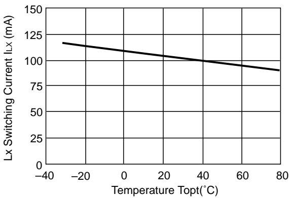
11) Lx Switching Current vs. Temperature
